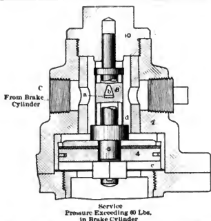
Fig. 2503. High-Speed Reducing Valve. Service Position.
